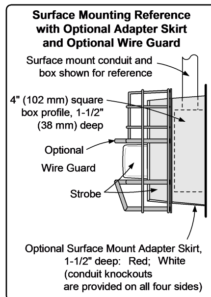
Figure 3: Wall Mount Installation Reference; Adapter Plate, Guard, and Adapter Skirt
