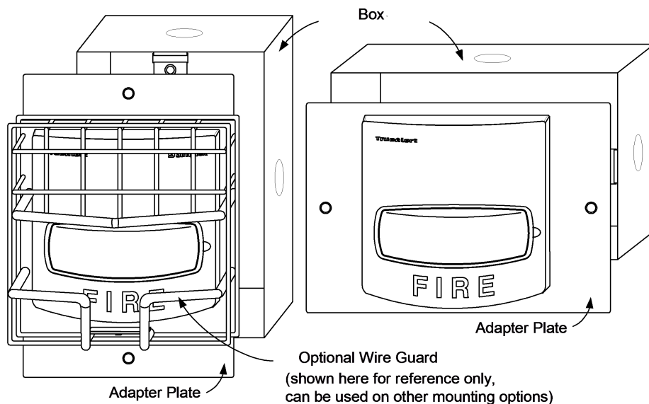
Figure 3: Wall Mount Installation Reference; Adapter Plate, Guard, and Adapter Skirt
