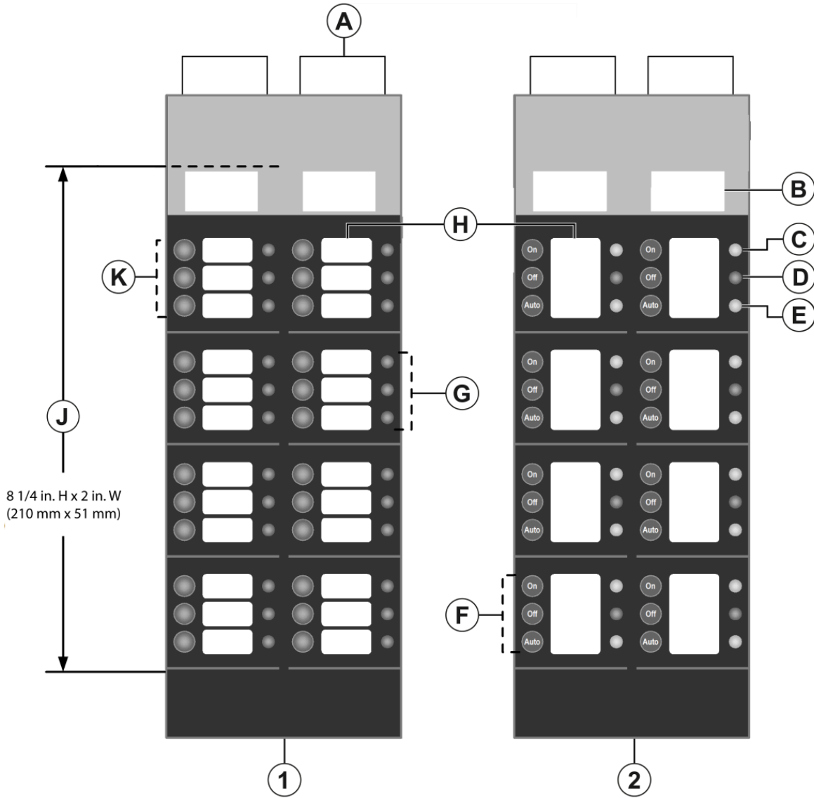
Figure 3: HOA and 24/24 LED/switch module detail reference
