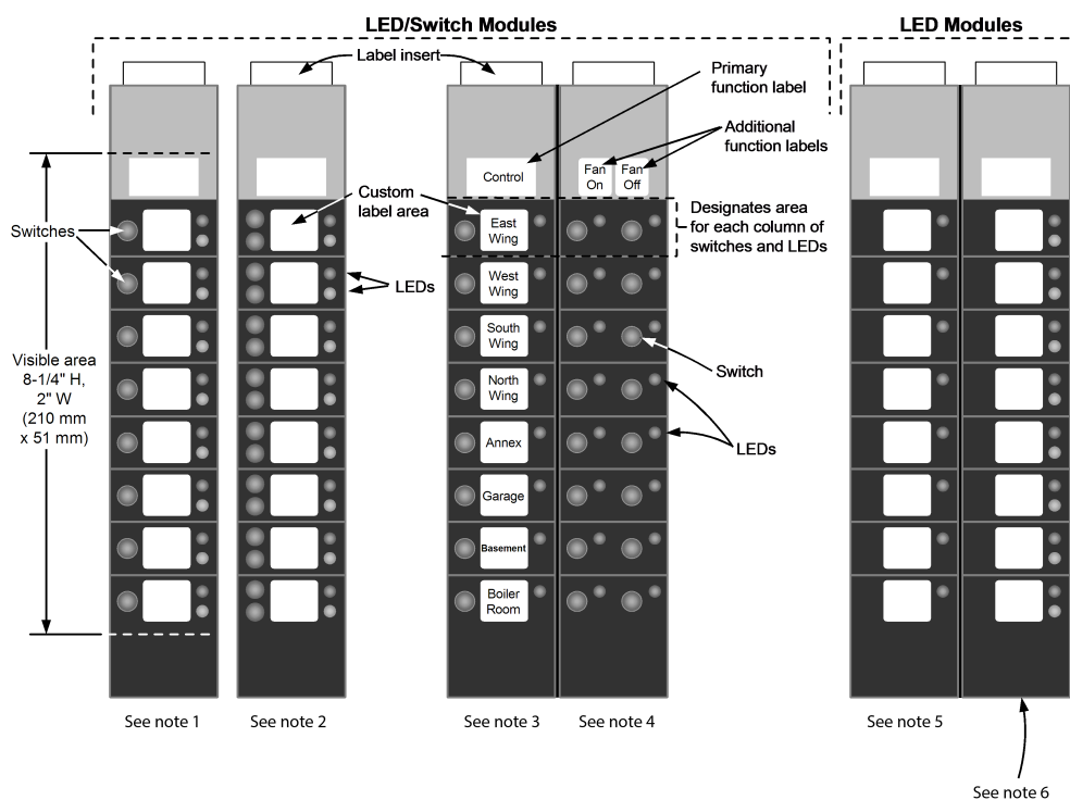
Figure 2: LED/Switch Module
