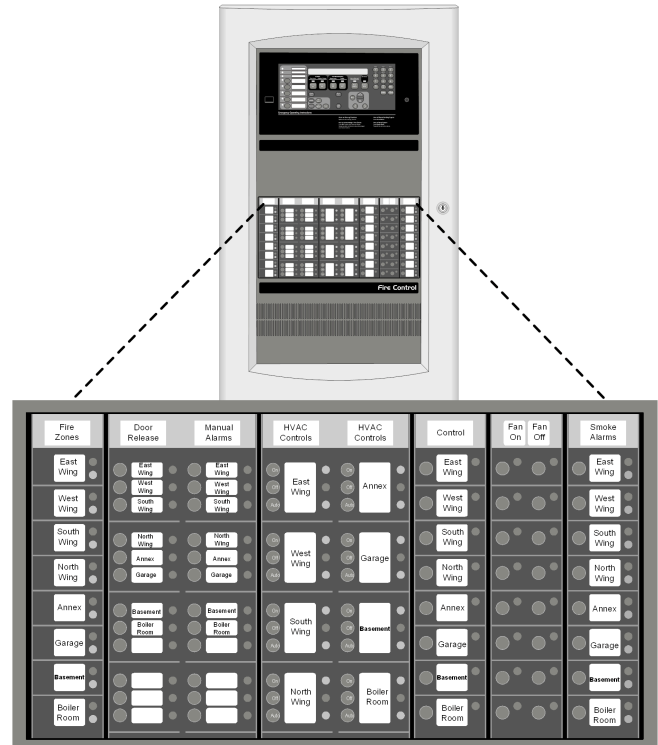
Figure 1: 4100ES 2-Bay Fire Alarm Control Panel with Sample of Available LED/Switch Modules
